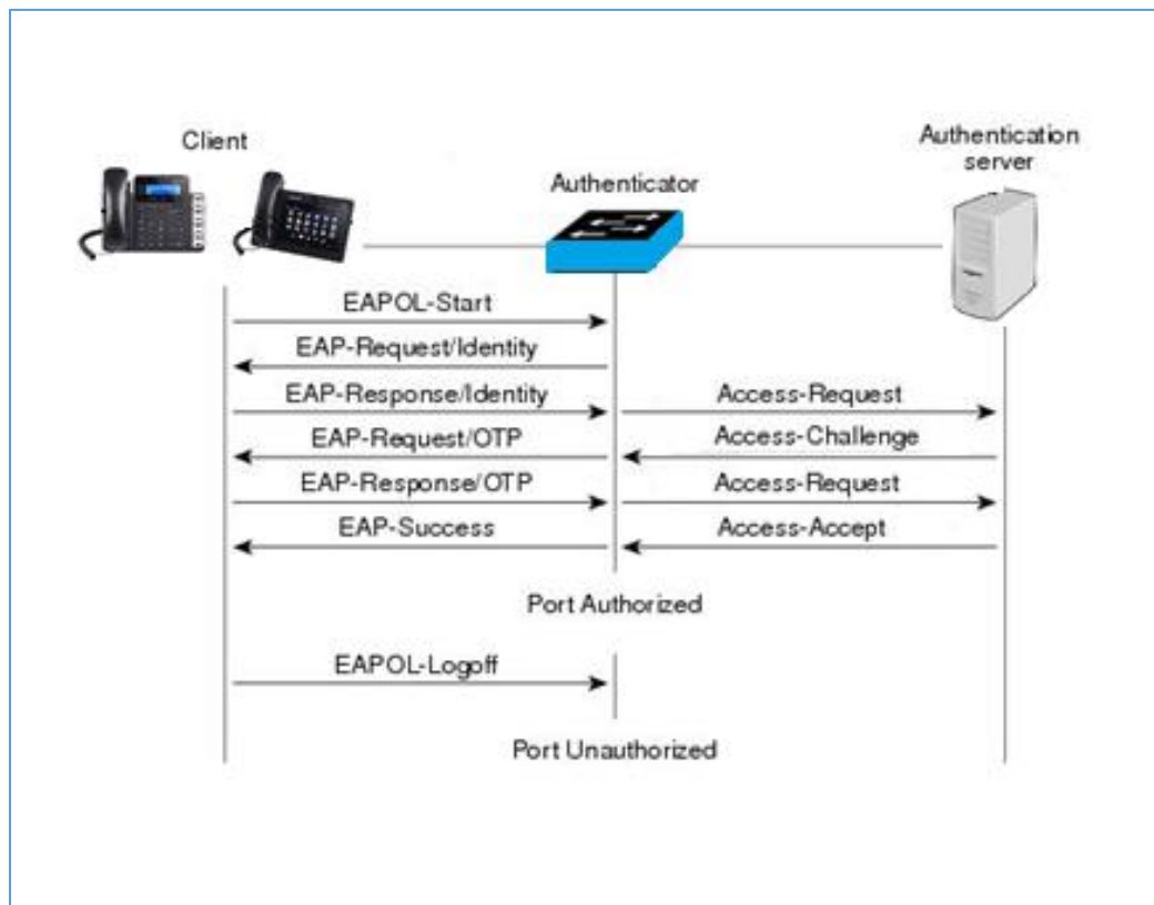
Figure 2: 802.1x Authentication Flowchart
