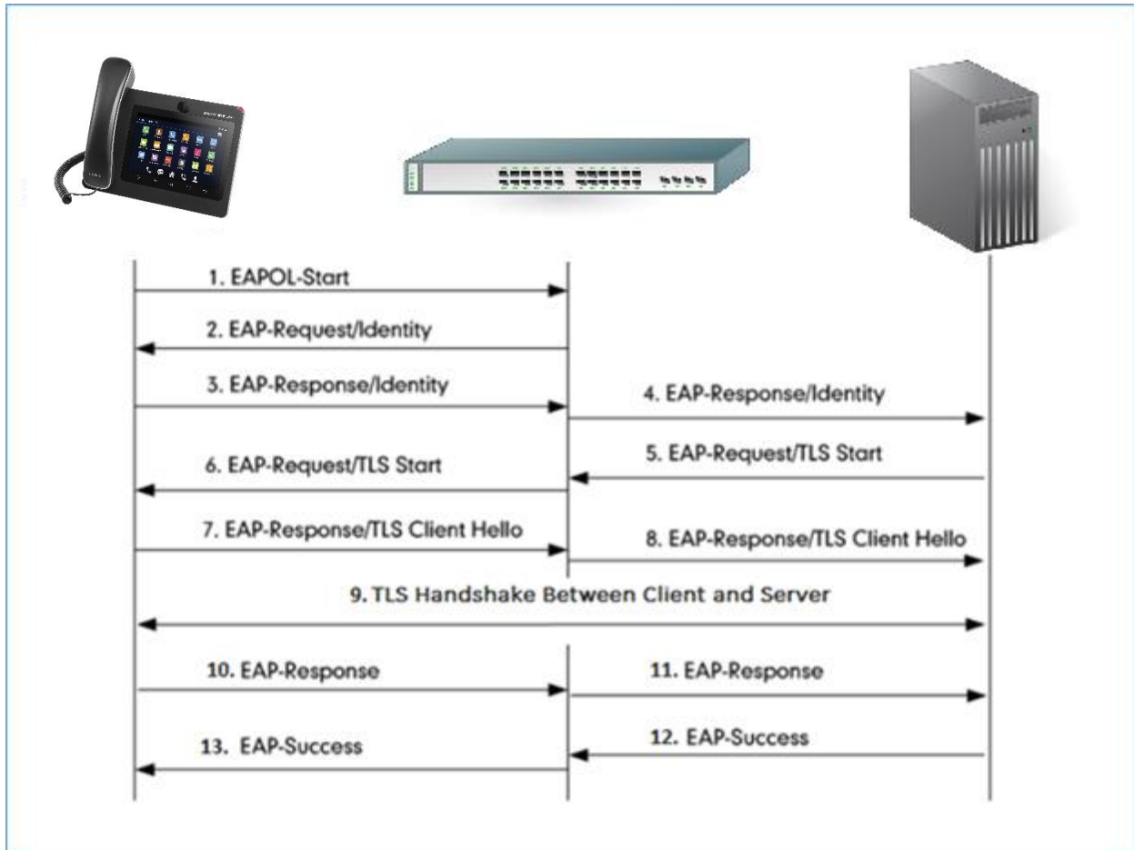
Figure 11: 802.1x Authentication Using TLS
