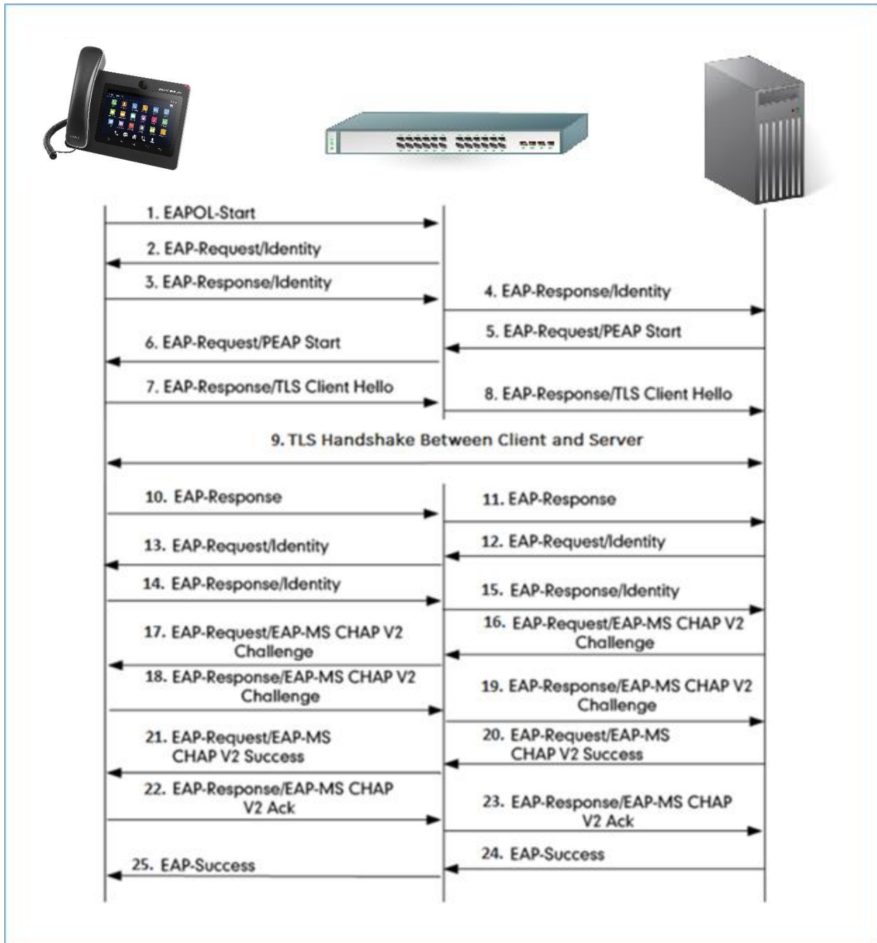
Figure 13: 802.1x Authentication Using PEAPv0/MSCHAPv2
