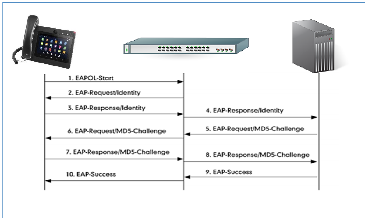
Figure 9: 802.1x Authentication Using MD5
