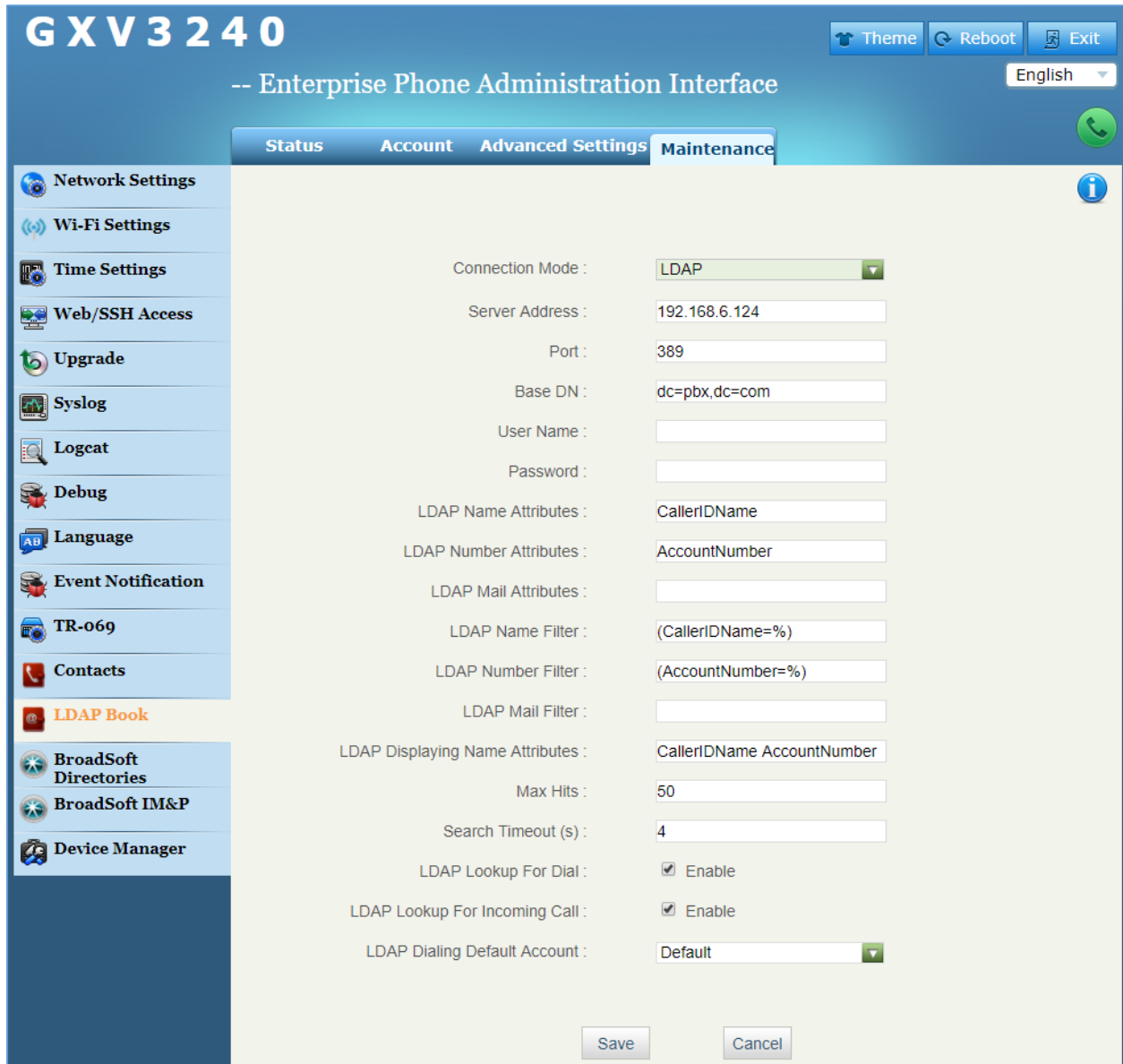
Figure 1: GXV3240 Web UI LDAP Settings
