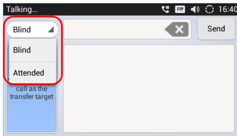
Figure 56: Attended Transfer
